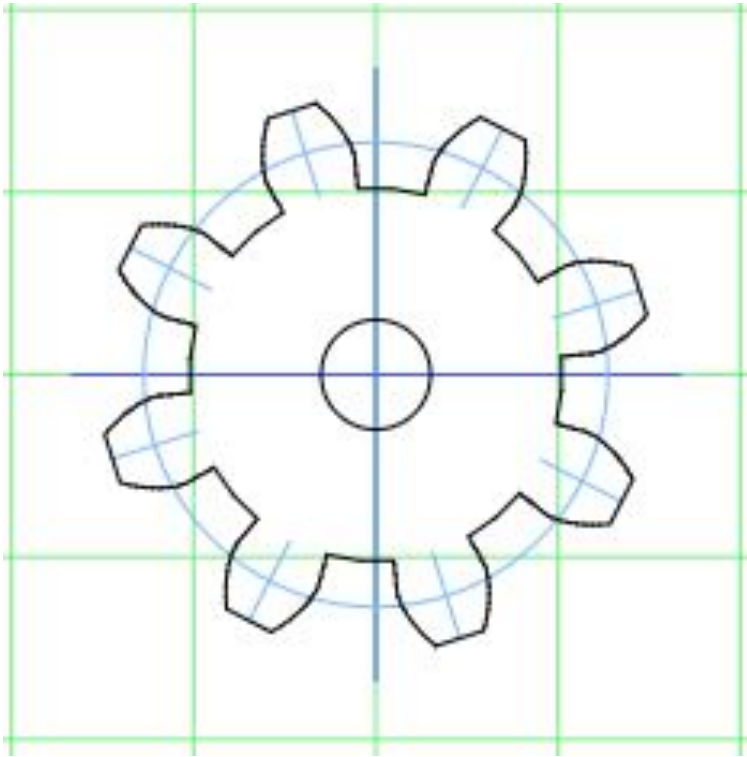
8 Teeth
